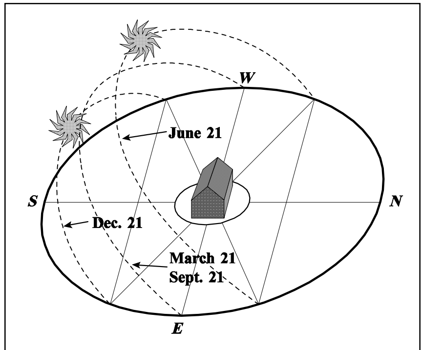
In northern latitudes, the sun is much lower in the sky in the winter than in the summer. For this reason, vertical glazing receives much more solar gain in the coldest part of the year. Sloped glazing takes in the most solar radiation in the summer.
